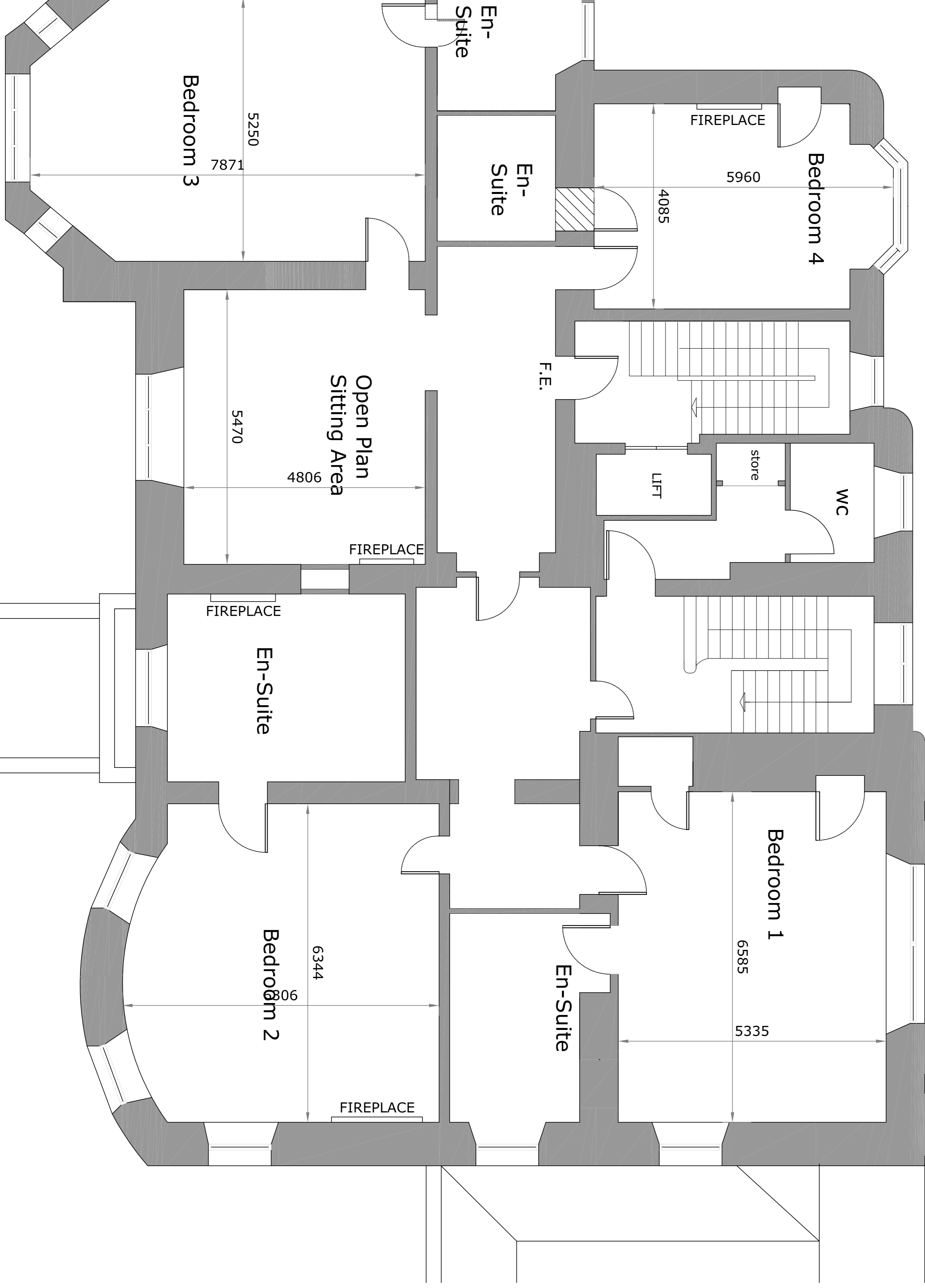
FIRST FLOOR PLAN 1:50 scale
